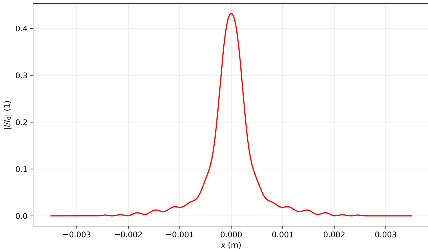
Intensity profile I(x, y = 0, z = 2.388)/I_0 , \text{Pin}=3.0\text{Pcr} , artificial time
